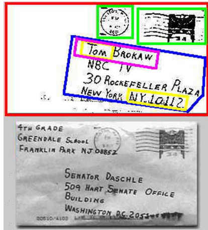
Figure 1. Wanda document annotation using regions. This picture of two envelopes from suspects in the recent anthrax criminal case provide us with an example of possible use of our WANDA regions: A region of interest is delineated, isolating one envelope from the page. A filter is applied to the region to clean the data. A hierarchy of regions (e.g. in address block, lines, words, and characters) is defined and annotated. Source: US Federal Bureau of Investigations.
